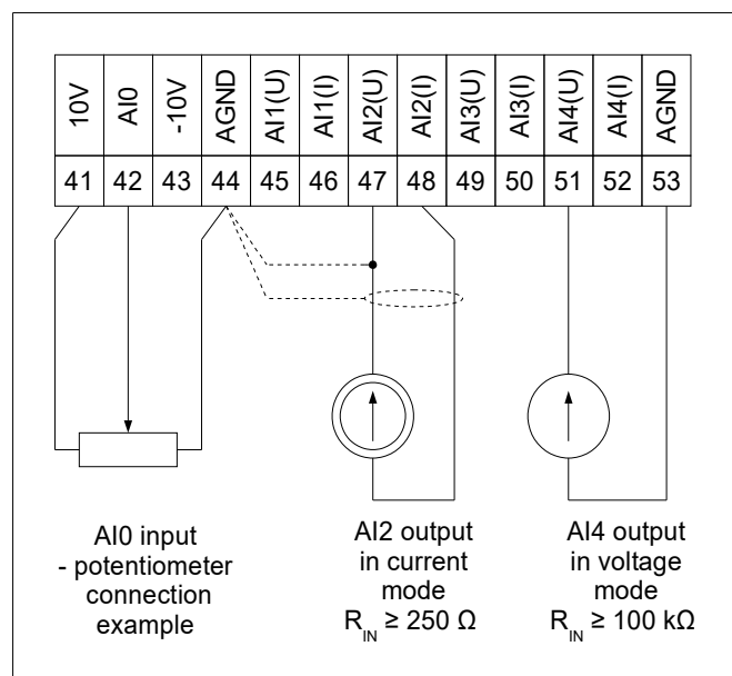
Fig. 4.7. An example of analog inputs connection; R_{IN} – internal resistance
