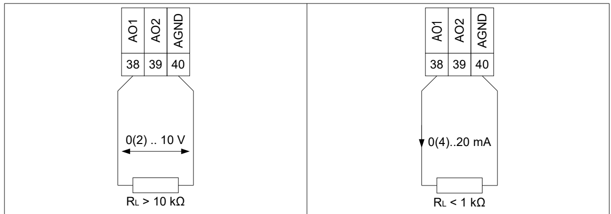
Fig. 4.5. AO1 output in voltage mode
