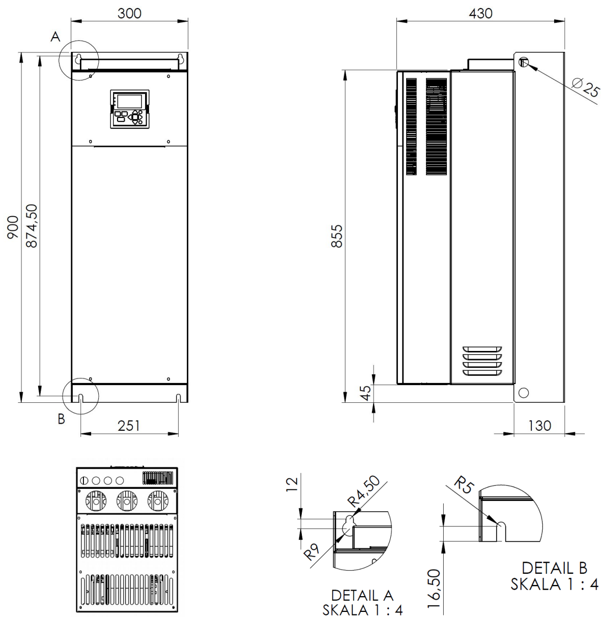
Fig. 3.2. Mechanical dimensions of MFC1000AcR frequency converters
