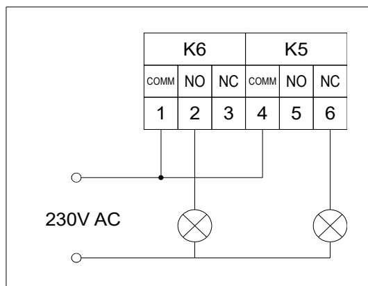
Fig. 4.3. An example of K5 and K6 relays outputs connection
