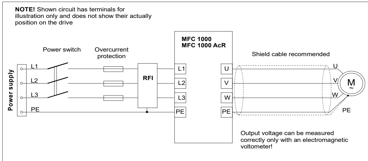
Fig. 4.1. Example connections of the power circuit
