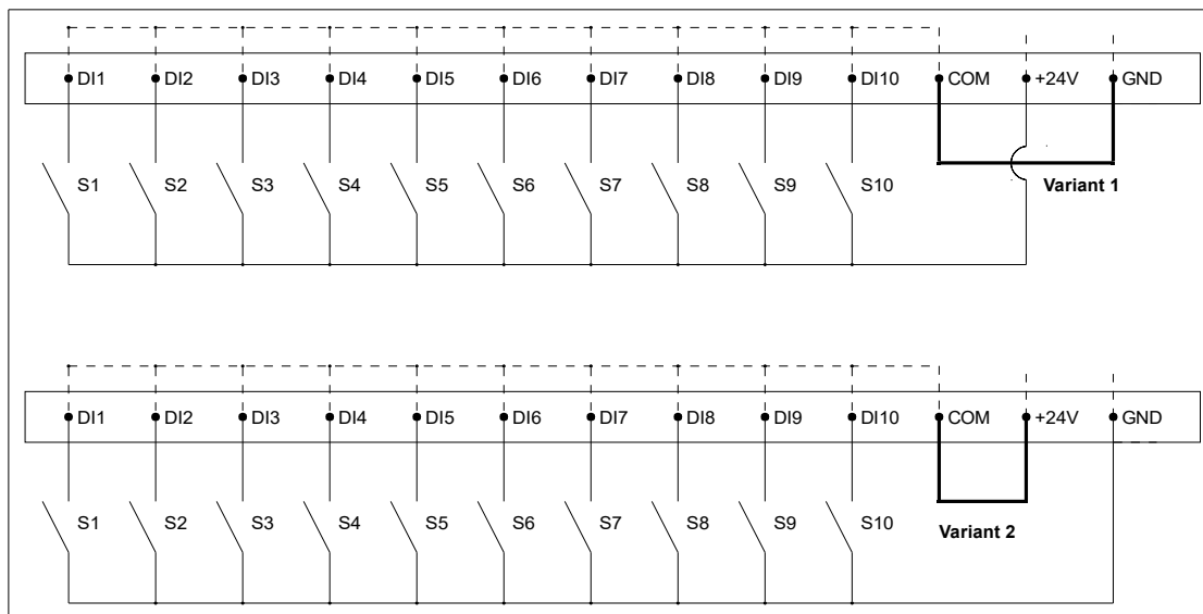
Fig. 4.4. Two variants of using the digital inputs: variant 1 and variant 2. The internal connections of the board are marked by a dashed line. S1 ÷ S10: exemplary connectors to switch on/off the digital inputs
